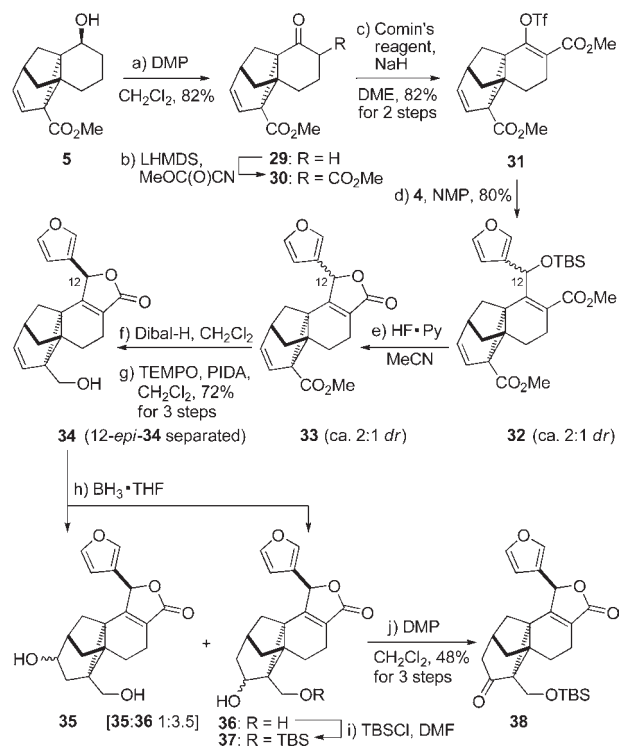
Scheme 4. Synthesis of Ketone 38 a
