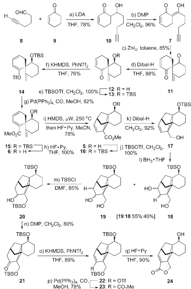
Scheme 2. Synthesis of Pentacyclic Hydroxy Lactone 24 a
