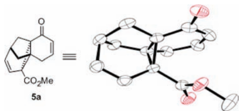
Figure 1. X-ray derived ORTEP representation of 5a . 11
