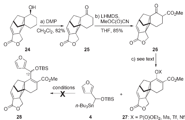
Scheme 3. Initial Attempts in the Installation of the Furanyl Moiety through Stille Coupling Engaging Enol Derivative 27 and Stannane 4 a
